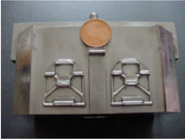
Pressure die casting mould Welding additive dia. 0,2
